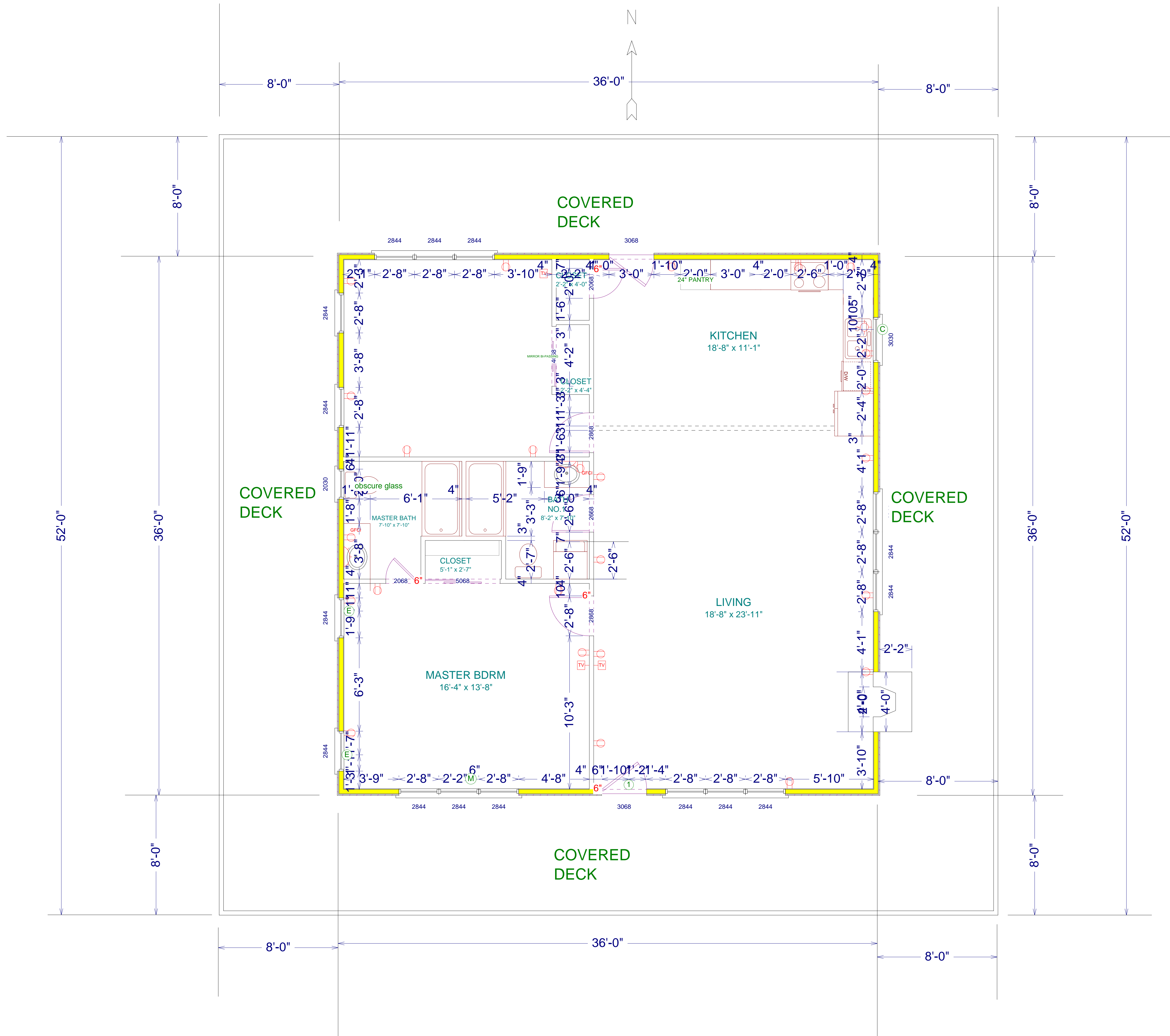
JORDAN CONSTRUCTION JCI SPEC. CABIN SH-15A FLOOR PLAN
